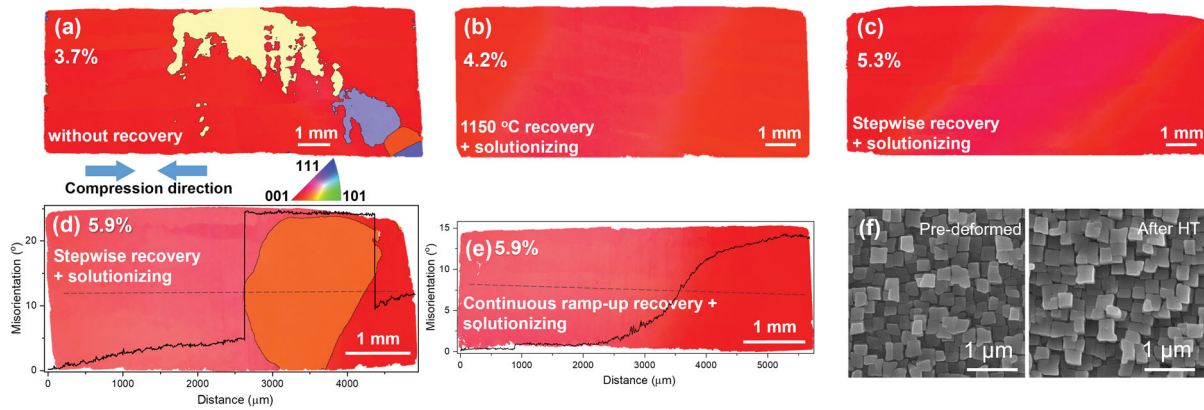
Figure 1. (a) to (e) Inverse pole figure (IPF) maps along the compression direction of the EBSD scanned cross-sections of specimens with various strain levels after recovery annealing and solutionizing treatment. (f) \gamma' morphologies before deformation and after heat treatment.
