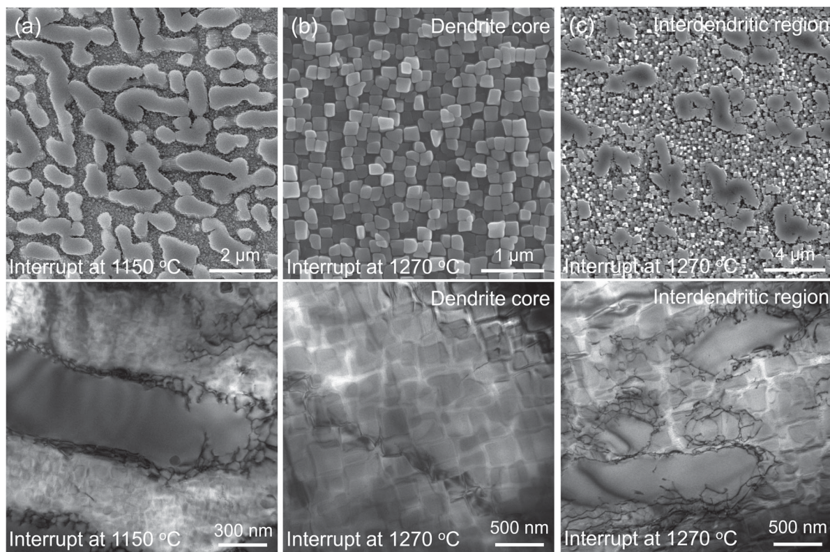
Figure 4. Microstructure of the specimen that was deformed to a plastic strain of 5.9% and then recovery annealed at high-temperature. (a) SEM and TEM characterization showing the evidence the coarsening of \gamma' -particles and formation of dislocation networks after annealing at 1150 °C. As the temperature is slowly ramped to 1270 °C, (b) dendrite cores are composed of uniform \gamma' -particles and almost no dislocations, while (c) low volume fraction of primary \gamma' -particles and low density of dislocations are observed in the interdendritic zones.
