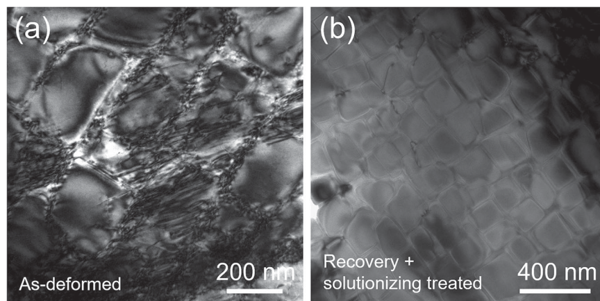
Figure 2. TEM observation of the dislocations in the 5.9% strained NBSC superalloy (a) before and (b) after recovery and subsequent solutionizing heat treatment.
