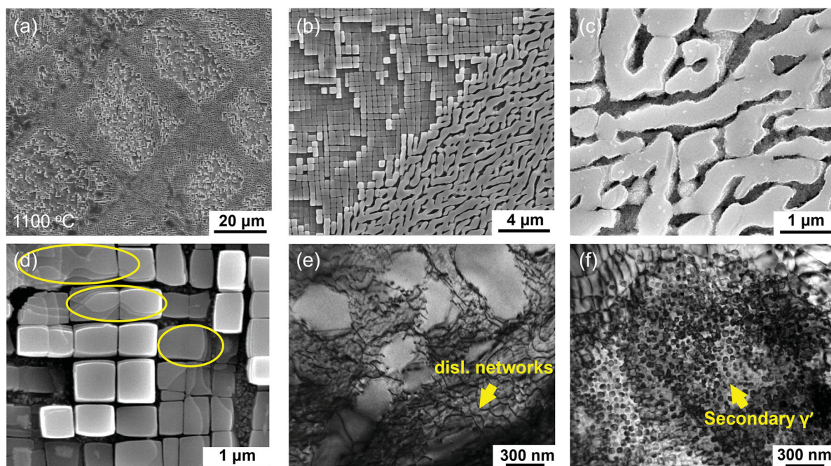
Figure 3. SEM and TEM characterizations of the specimen that was deformed and then subjected to recovery annealing at 1100 °C. Grid-like structures observed at (a) low and (b) high magnification in SEM. Morphologies of the (c) coarsened and (d) cuboidal \gamma' in the dark and bright contrast regions of (a), respectively. TEM image of the (e) coarsened \gamma' surrounded by dislocation networks at the \gamma/\gamma' interphase while the (f) secondary \gamma' rich regions are almost dislocation-free.
